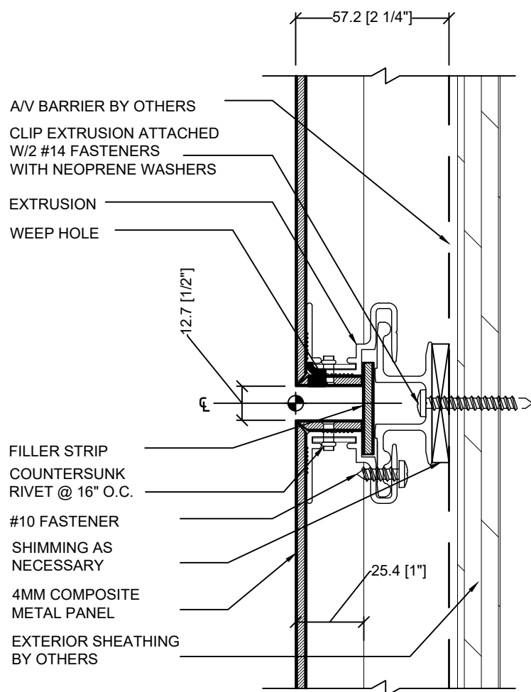
HORIZONTAL JOINT TYP.
